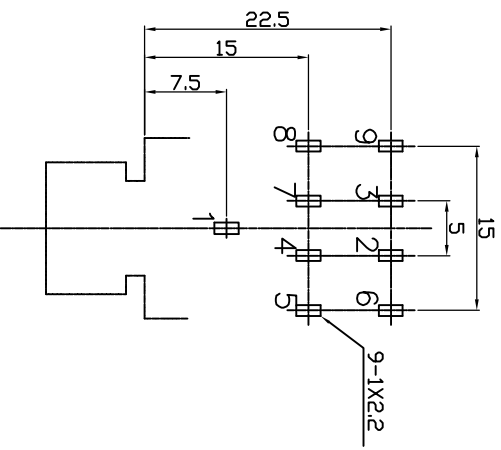
PCB Holes Diagram Top View
